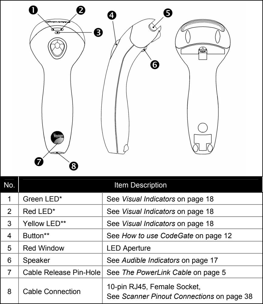
Figure 1. Scanner Components
